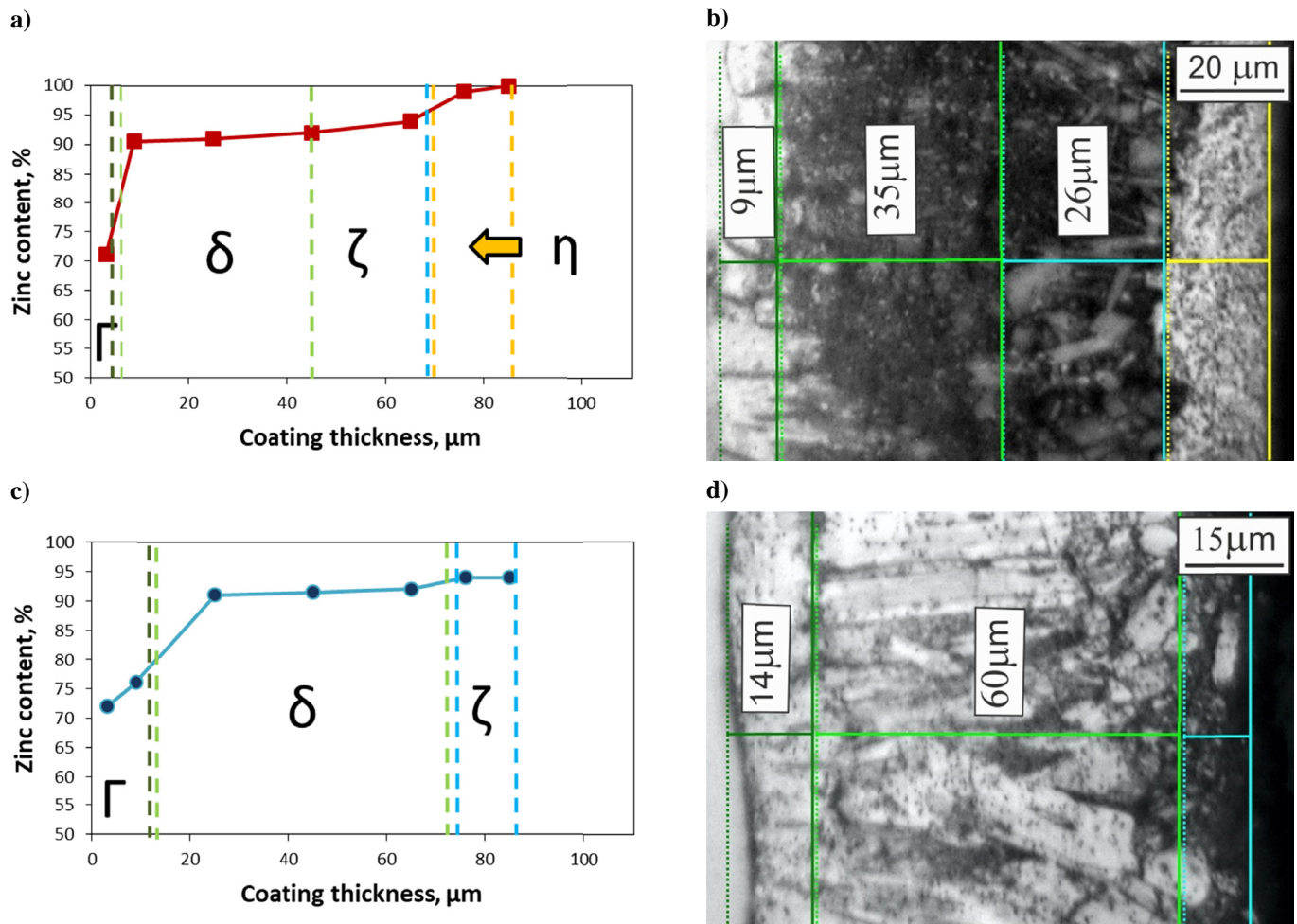
Fig. 8. The Zn distribution at the coating cross section deposited on bolt head before (a) and after HT (c) compared to coating microstructure: b – without HT; d – after HT in 430^\circ\text{C}
