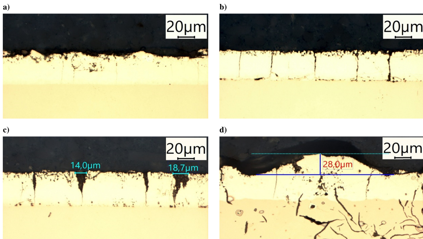
Fig. 3. The microstructure observed at the cross section of zinc coating deposited on steel after the HT – a (430°C), b (460°C), c (530°C) and cast iron – d (530°C)
