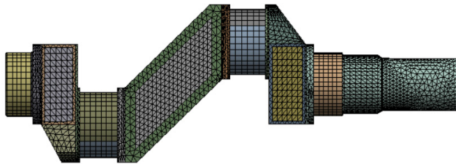
Fig. 7. Grid scheme for the crankshaft model
