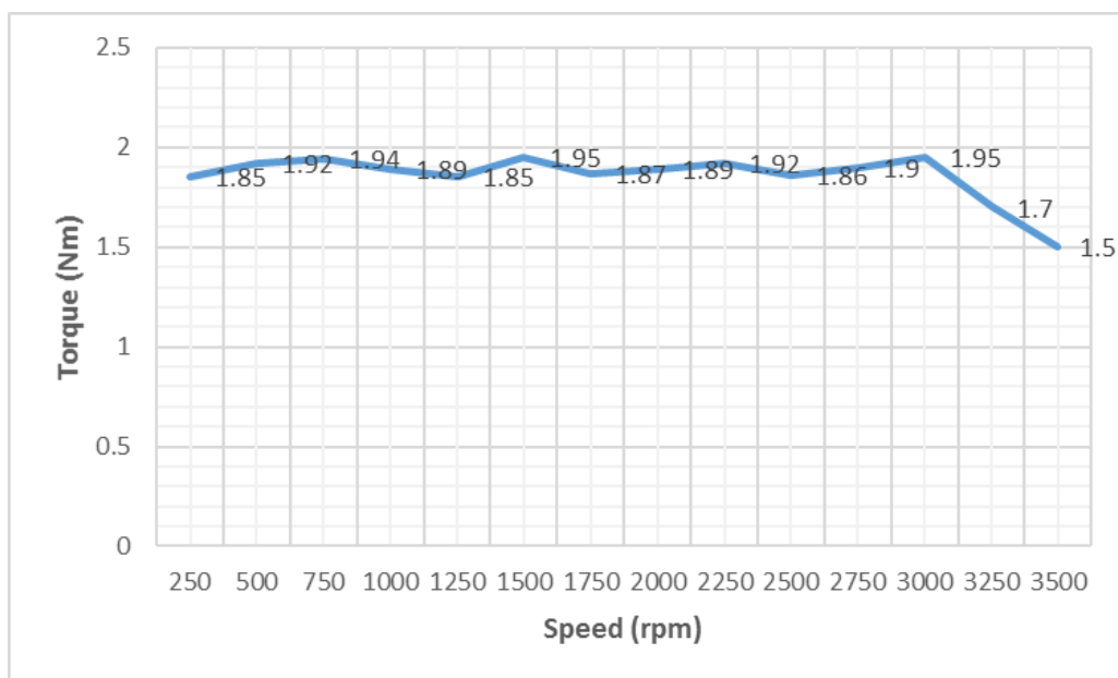
Fig. 16 HTPMSM: IPM: Speed-Torque Characteristics at Rated Loaded Conditions
