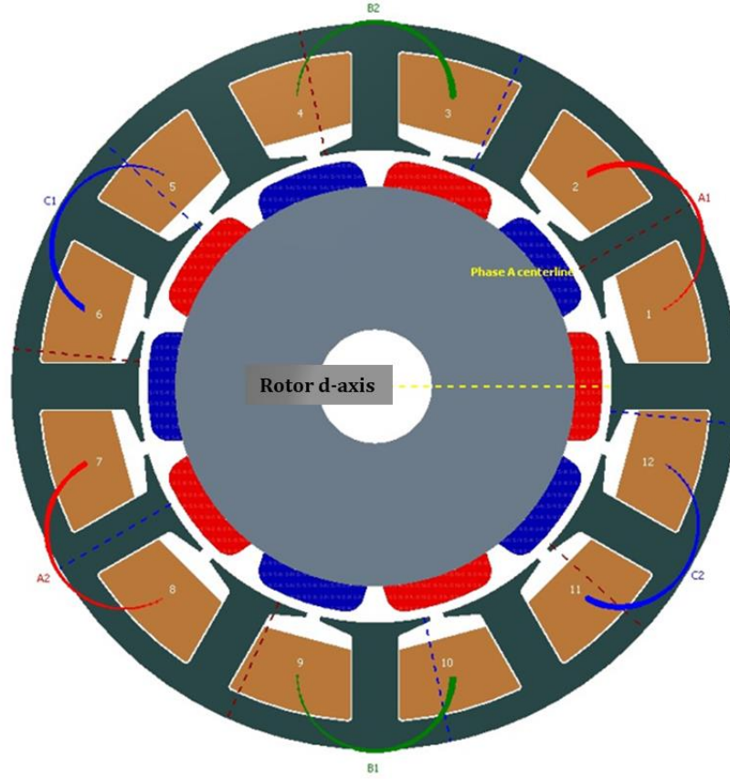
(a) Stator and Rotor Configuration
