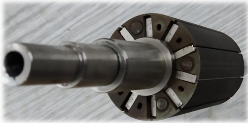
Fig. 13 HTPMSM: IPM Type: Rotor
