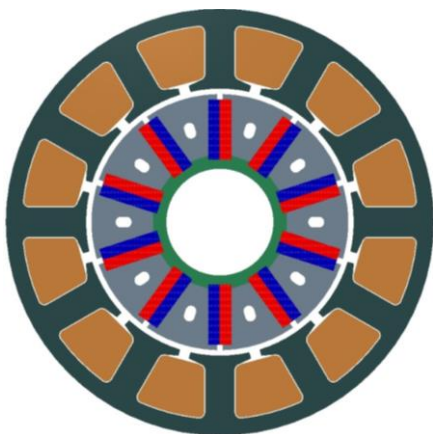
(a) Stator/Rotor Configuration Fig. 8 HTPMSM: IPM Type: Spatial Plots
