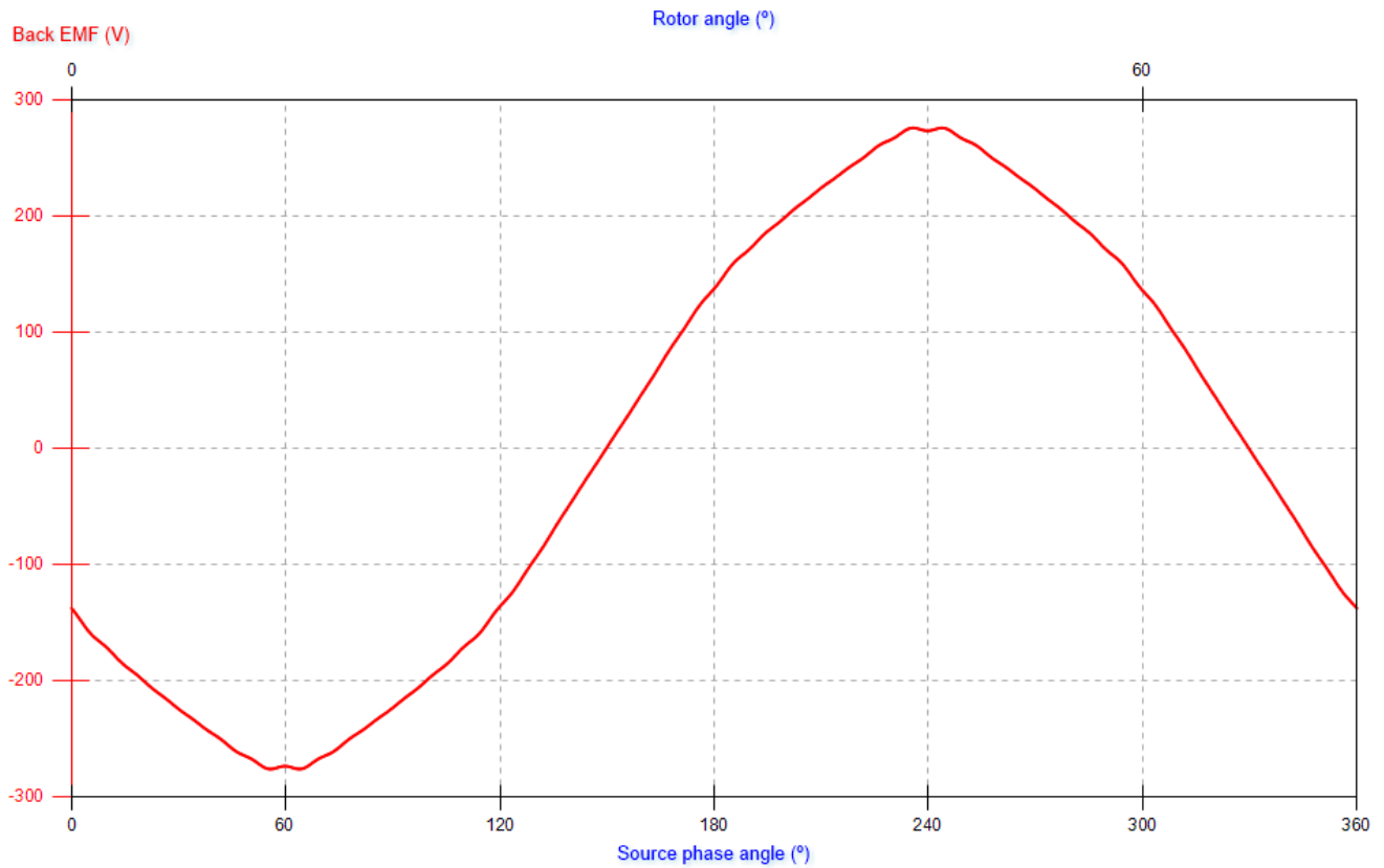
Fig. 3 HTPMSM: SPM Type: Back EMF @ 3000 rpm
