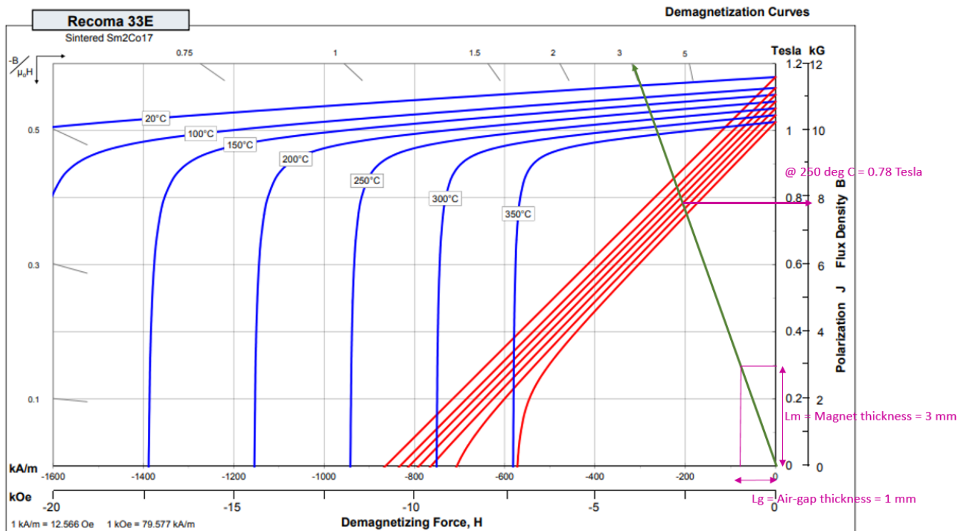
Fig. 17 Demagnetization characteristics of the Sm 2 Co 17 Magnet
