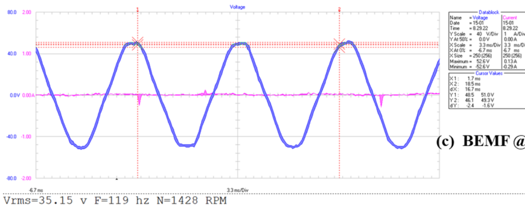
Fig. 14 Line-Line BEMF Voltages of HTPMSM IPM Type Rotor
