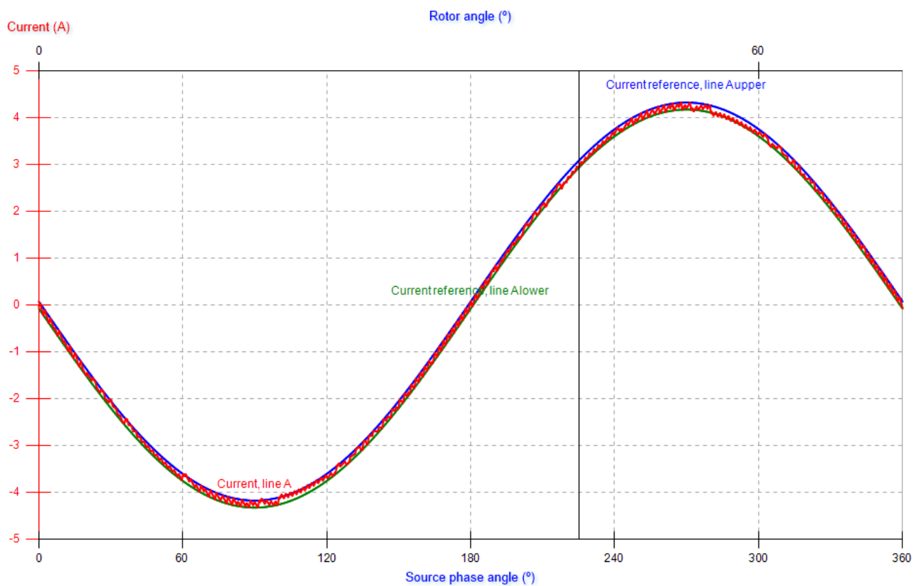
Fig. 4 HTPMSM: SPM Type: Phase Current
