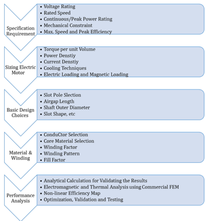
Fig. 1 Design Methodology of HTPMSM
