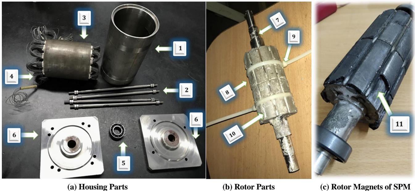
1. Inconel Stator Housing, 2. Studs, 3. Vanadium Cobalt Iron Laminations for Stator, 4. Stator Core with Ceramic Coated Winding 5. Nichrome Coated Bearings, 6. Front & Back Flange Mount Inconel, 7. Inconel Shaft, 8. Recoma Grade Samarium Cobalt Magnet 9. Cable Tie, 10. High Temperature Adhesives – Aremco, 11. Breakdown of Rotor Magnets
