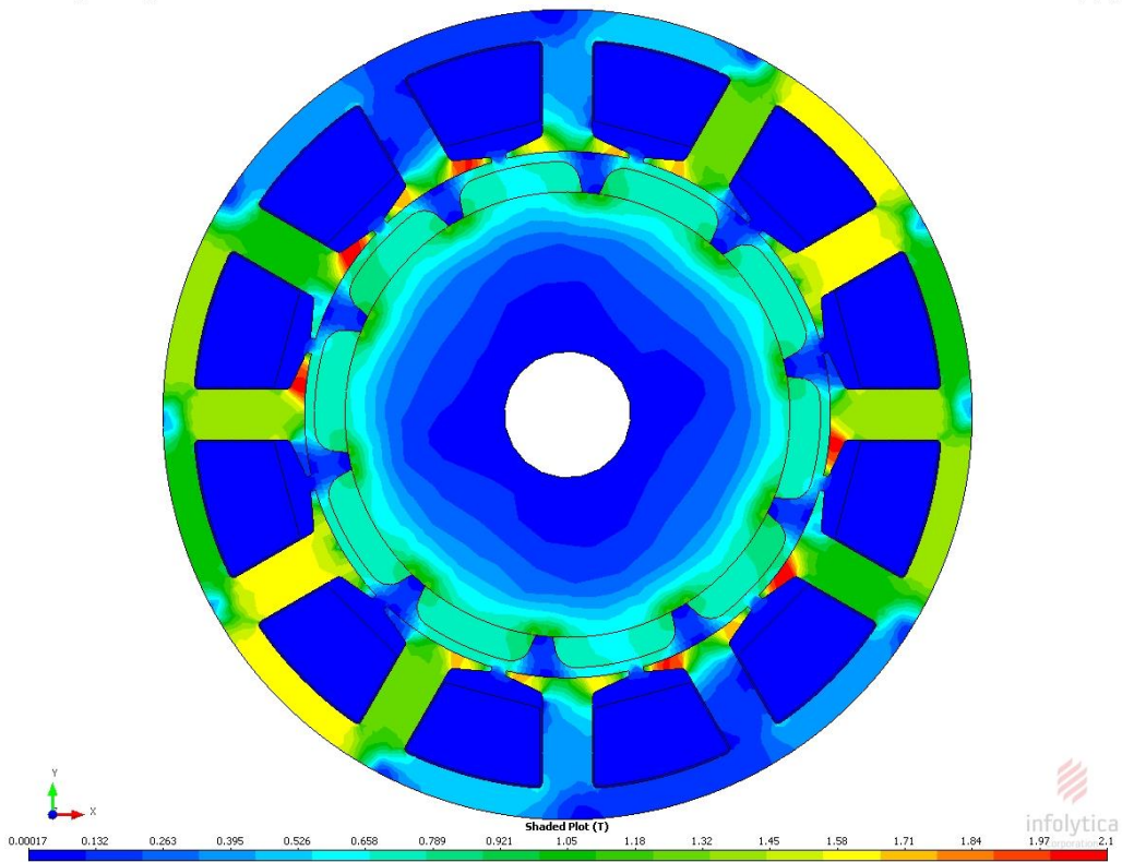
(b) Instantaneous Flux Density Fig. 2 HTPMSM: SPM Type: Spatial Plots
