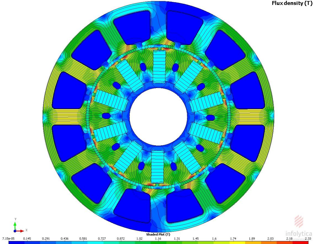
(b) Instantaneous Flux Density Fig. 8 HTPMSM: IPM Type: Spatial Plots
