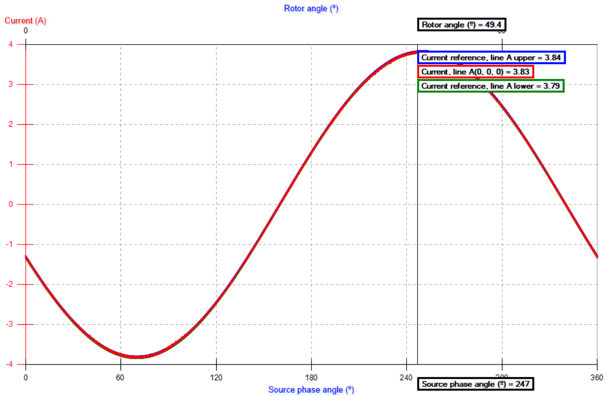
Fig. 10 HTPMSM: IPM Type: Phase Current
