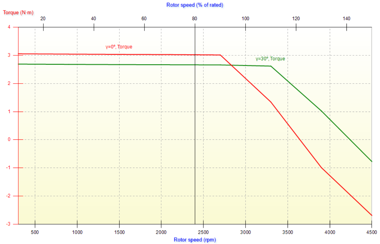
Fig. 11 HTPMSM: IPM Type: Speed – Torque Characteristics
