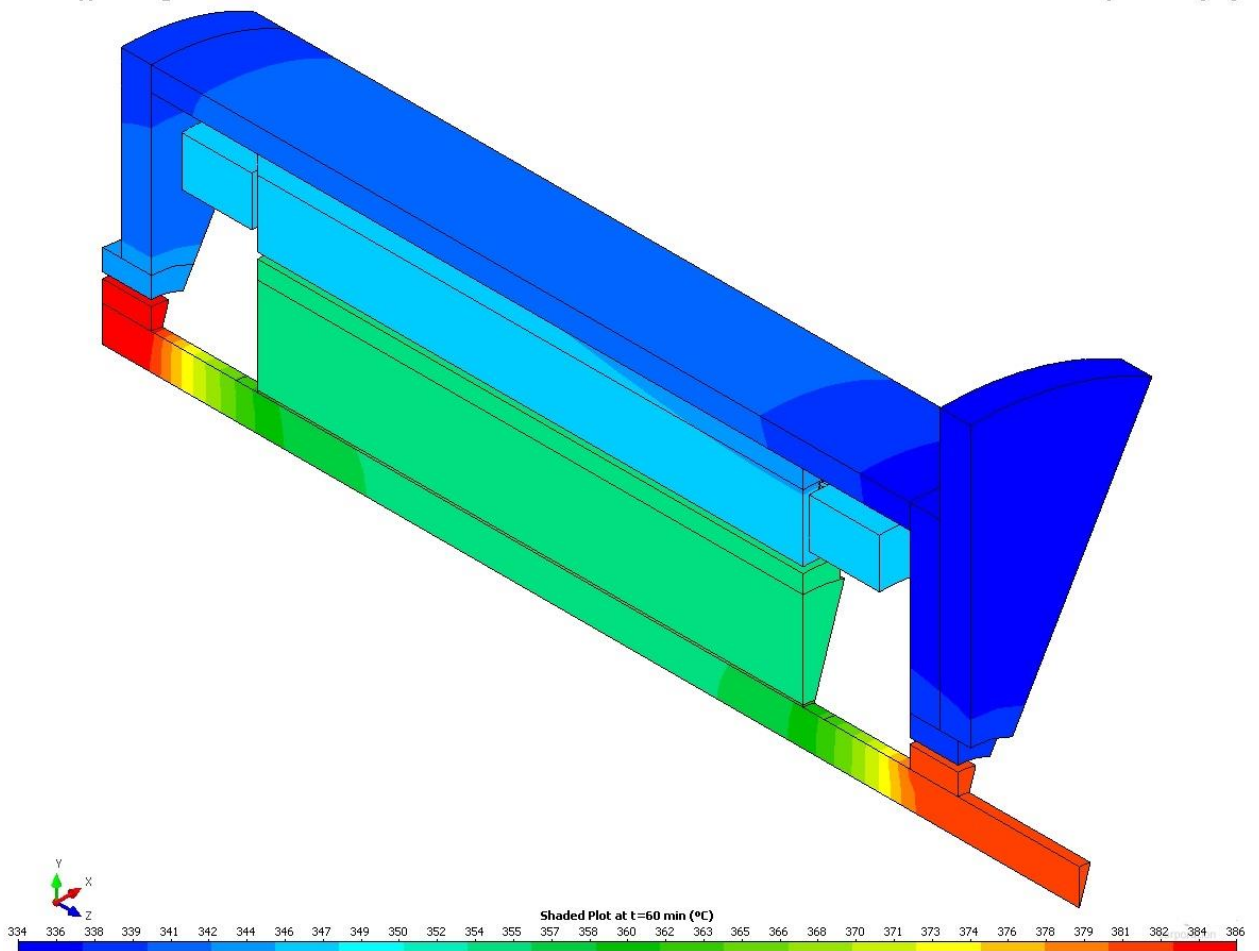
Fig. 6 HTPMSM: SPM Type: Thermal Fields
