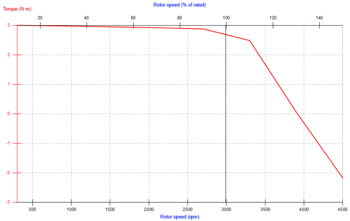
Fig. 5 HTPMSM: SPM Type: Speed – Torque Characteristics
