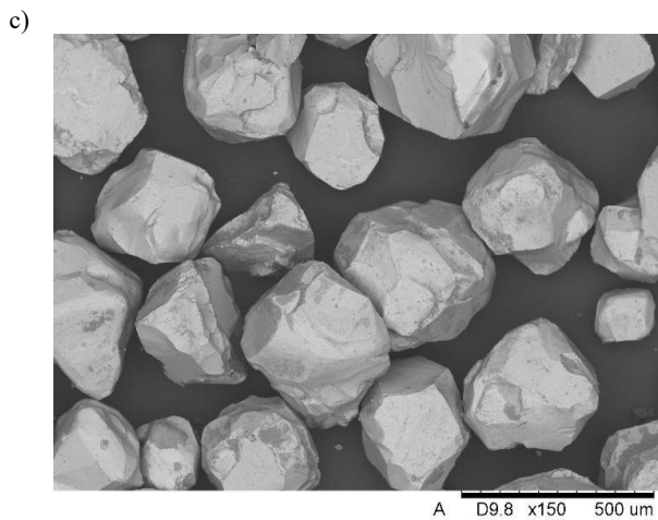
Fig. 1. Surface topography of sand grains: quartz (a), olivine (b), chromite (c), SEM (magnification x150)
