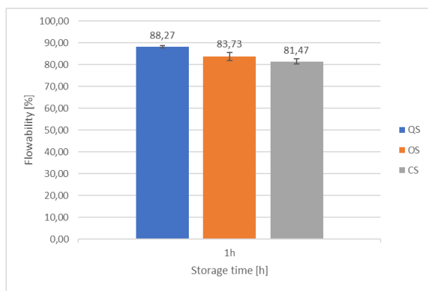
Figure 3. Results of measurements of the flowability of moulding sands depending on the type of matrix
