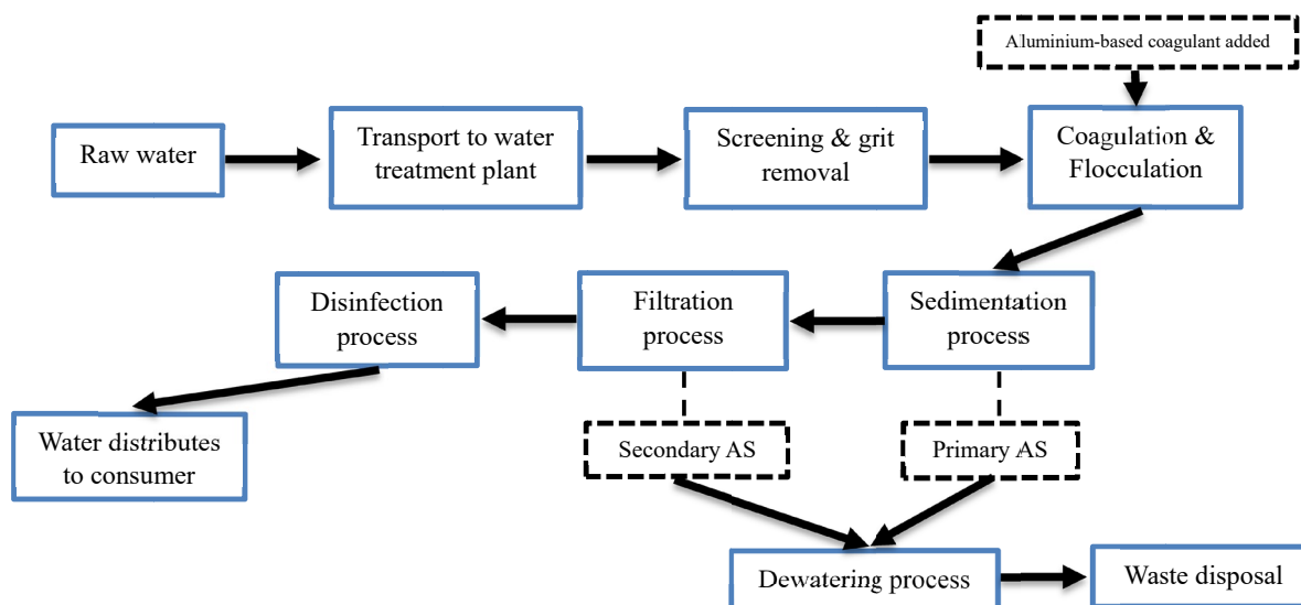
Fig. 2. The conventional treatment of drinking water process [35-37]
