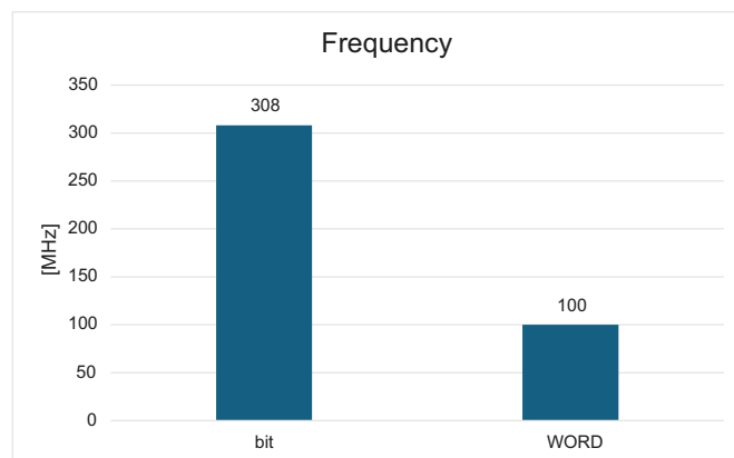
Fig. 11. Max frequency of bit and WORD RISC-V cores
