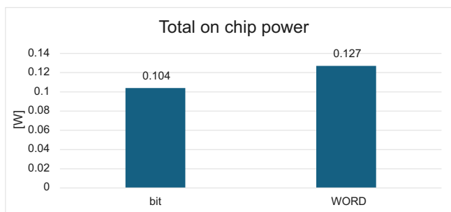
Fig. 9. Power analysis of the bit and WORD RISC-V cores
