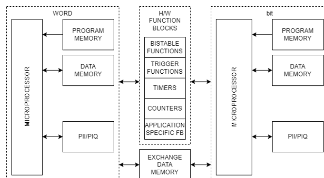
Fig. 3. The idea of the bit.WORD programmable logic controller
