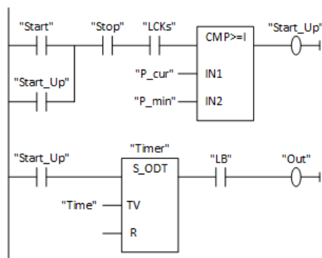
Fig. 2. LD control program
