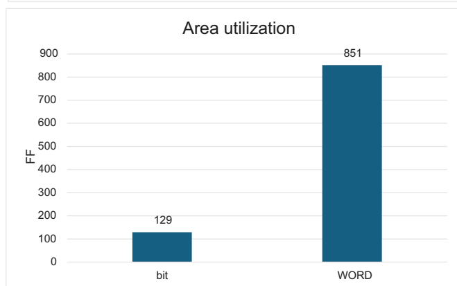
Fig. 10. Area analysis of the bit and WORD RISC-V cores
