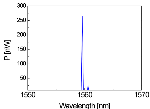
Fig. 7. Lasing action in a silica microsphere of 150 μm in diameter coated by a film of composition 70SiO 2 -30HfO 2 activated with 0.3% mol Er 3+
