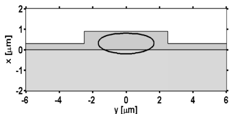
Fig. 2. a) SEM microphoto of a channel waveguide obtained by a dry-etching process on 70SiO 2 -30HfO 2 planar waveguide fabricated by sol-gel route; b) schematic cross section of the rib silica-hafnia waveguide showing the 2/3 mode intensity contour after Ref. 23
