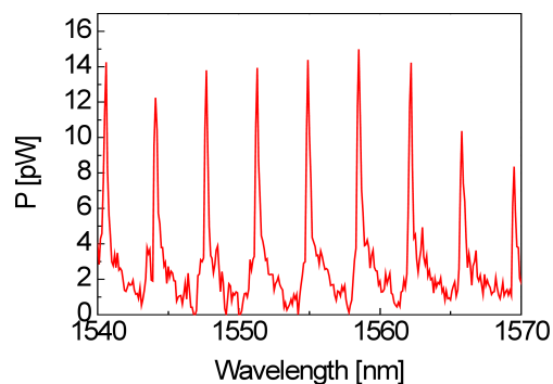
Fig. 6. The WGM luminescence of a silica microsphere of 150 μm in diameter coated by a film of composition 70SiO 2 -30HfO 2 activated with 0.3% mol Er 3+
