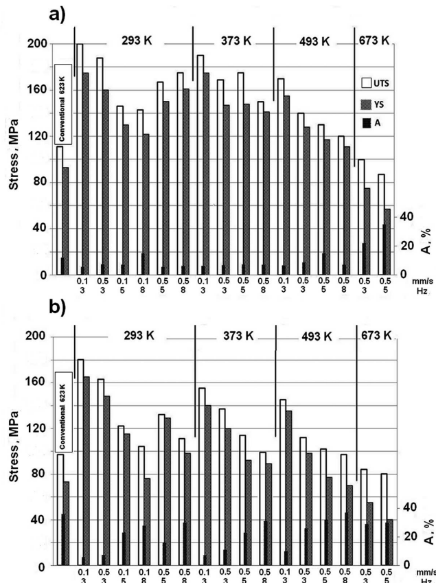
Fig. 1. Mechanical properties of aluminum wire extruded by means of KoBo method: (a) beginning part of the extrudate, (b) ending part of the extrudate. Initial temperature of extruded billet, velocity of the punch displacement, oscillation frequency is marked in the figure
