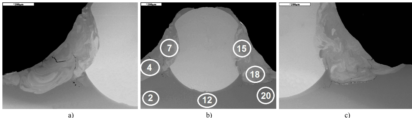
Fig. 5. Views of variant B joints, a) and c) left and right sides, respectively (magnification 200x), b) microhardness measurement points (magnification 75x)
