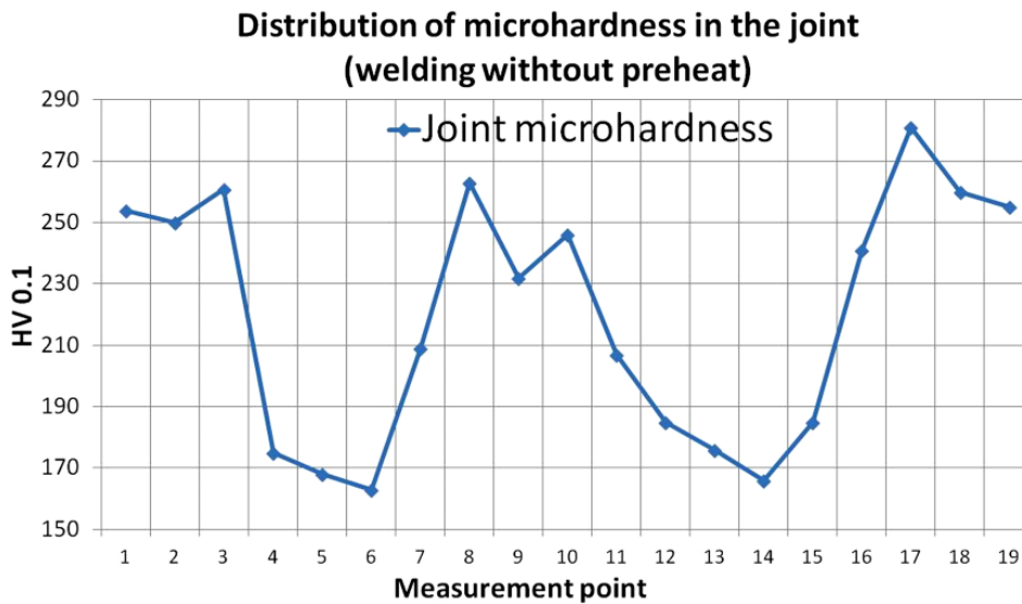
Fig. 4. Distribution of microhardness of a variant A joint, according to Fig. 2b
