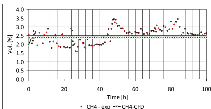
Fig. 8. Changes in the concentration of CH 4 in the time interval of 100 hours of coal gasification process, obtained from the solution of the CFD numerical model and measurements on the experimental model in EM “Barbara”
