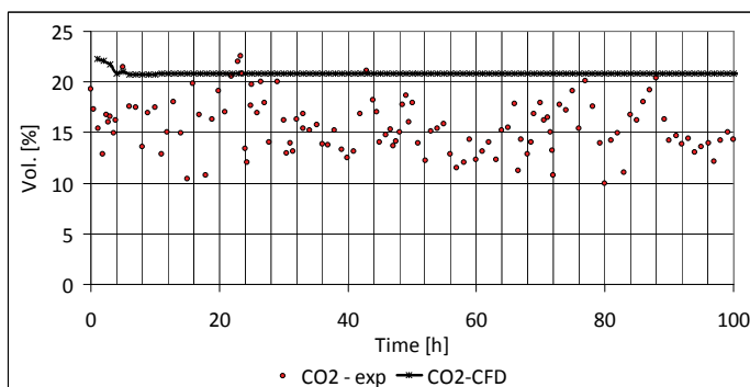
Fig. 9. Changes in the concentration of CO 2 in the time interval of 100 hours of coal gasification process, obtained from the solution of the CFD numerical model and measurements on the experimental model in EM “Barbara”
