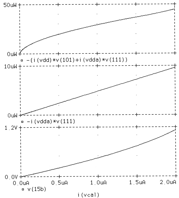
Fig. 6. Simulated DC properties at the linear output of the neuron driven by three synapses of the type shown in Fig. 3. a) power consumed by the whole circuit (neuron plus three synapses), b) power consumed by the neuron only, c) the linear output voltage, V_{O2} , of the neuron versus its input current I_{IN}
