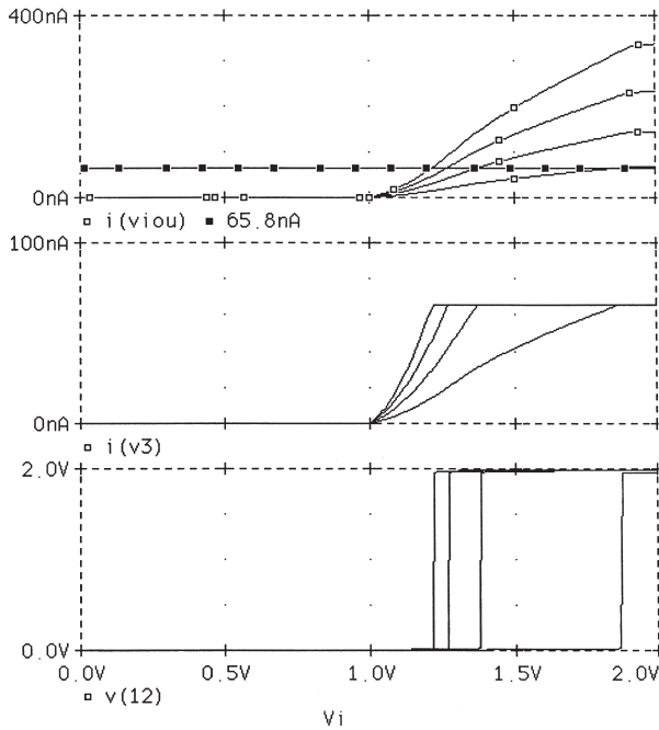
Fig. 4. The neuron basic signals for V_{th} = 0.49 V when driven by one synapse: a) input current I_{IN} for four synapse weights versus input voltage V_I of the synapse, b) drain current I_{M3} of the transistor M03 versus V_I , c) V_{O1} voltage at the step output versus V_I
