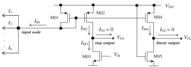
Fig. 1. Simple transresistance CMOS neuron with step and linear activation function outputs
