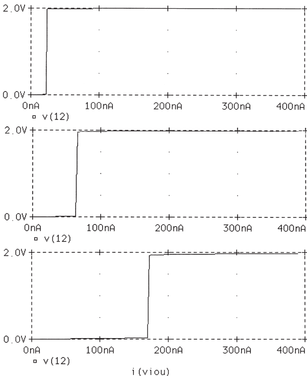
Fig. 5. Transfer characteristics concerning the step output of the transimpedance neuron showing the possibility of controlling the threshold current I_{th} by means of V_{th} : a) V_{O1} versus I_{IN} for V_{th} = 0.48 V (upper plot), b) V_{O1} versus I_{IN} for V_{th} = 0.49 V (middle plot), c) V_{O1} versus I_{IN} for V_{th} = 0.505 V (bottom plot)
