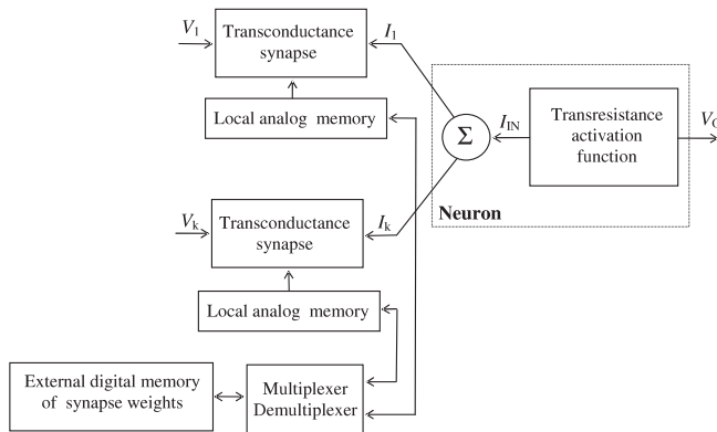
Fig. 2. Static neuron model including synapses coupled with local memories suitable for adaptive ANN's implemented in a chip form and trained on silicon
