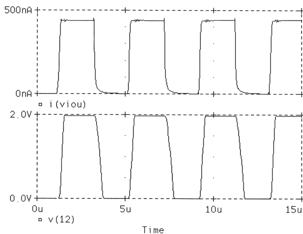
Fig. 7. Time response at the neuron step output: a) input current I_{IN} versus time (upper plot), b) output voltage V_{O1} versus time (bottom plot)
