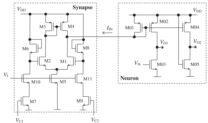
Fig. 3. Implemented in 0.35 \mu\text{m} CMOS process neuron with one synapse tested in the way of simulations
