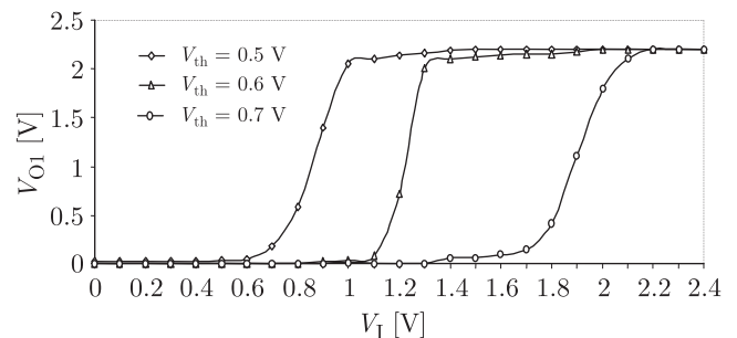
Fig. 8. Measured transfer characteristic (output voltage V_{O1} versus V_I voltage at the synapse input) of the circuit shown in Fig. 3, for V_{th} equal to 0.5 V, 0.6 V and 0.7 V
