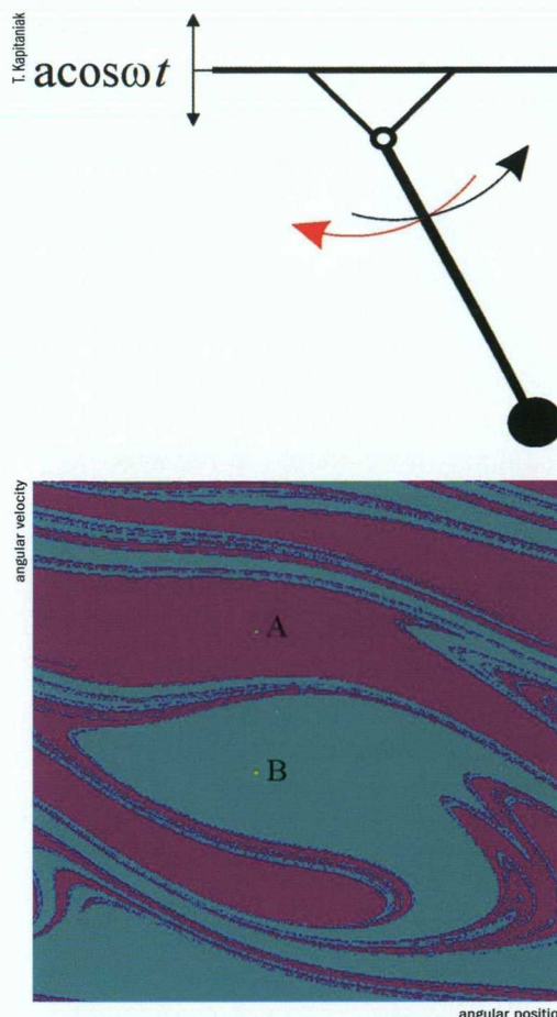
Figure 3: the setup of an externally excited pendulum (above) and the attraction basins of its attractors in the space of initial states (below)
