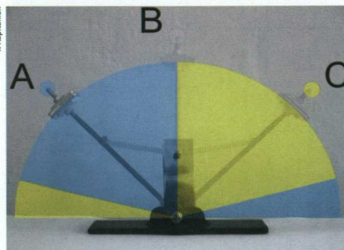
Figure 1: An inverted pendulum and the attraction basins of its attractors: if the initial state is in the blue areas, the system will eventually come to rest at point A (initial states in the yellow areas tend to develop towards point C)
