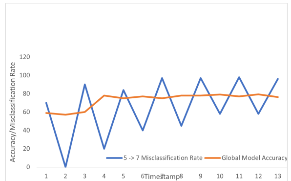
Fig. 7. Accuracy/Misclassification Rate of Attack
