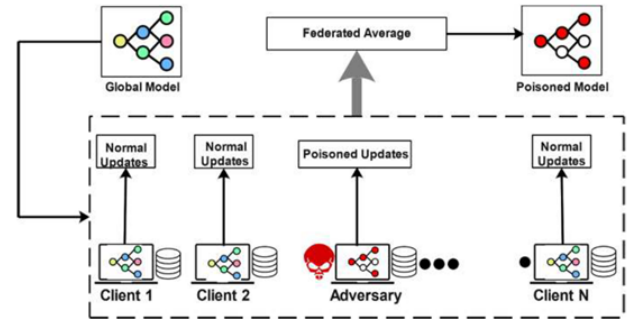
Fig. 2. Federated learning with label-flipping attacks
