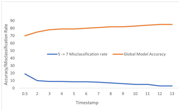
Fig. 8. Accuracy/Misclassification Rate of Attack when Attack is enabled
