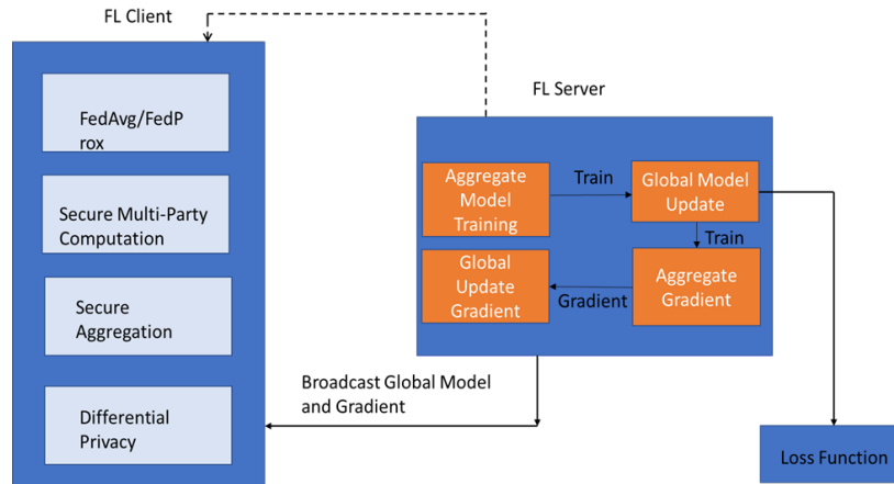
Fig. 1. Architecture of proposed FedAssess framework
