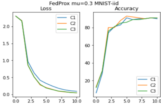
Fig. 5. Loss and Accuracy of FedProx
