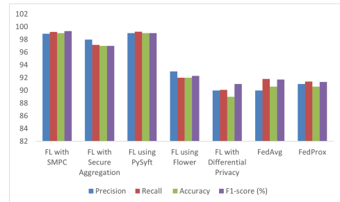
Fig. 4. Comparison based on evaluation metrics
