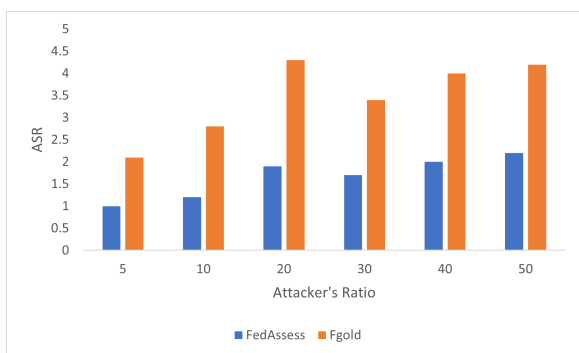
Fig. 9. Analysis of Attack Success Rate
