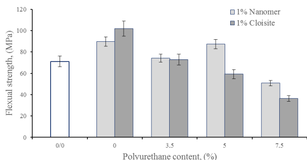
Figure 6. Effect of polyurethane content on the flexural strength of epoxy resin modified with 1 wt% Nanomer or 1 wt% Cloisite
