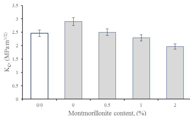
Figure 8. Effect of montmorillonite (Cloisite) content on the critical stress intensity factor ( K_C ) of the epoxy matrix modified with 1 wt% Nanomer
