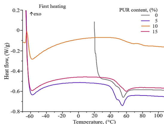
Figure 11. DSC thermograms of epoxy resin modified with different amounts of polyurethane
