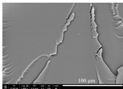
Figure 13. SEM micrograph of unmodified epoxy matrix
