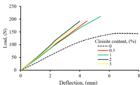
Figure 3. Load-deflection curves of epoxy resin modified with different amounts of Cloisite
