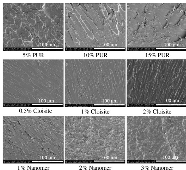
Figure 14. SEM micrographs of modified epoxy resin modified
