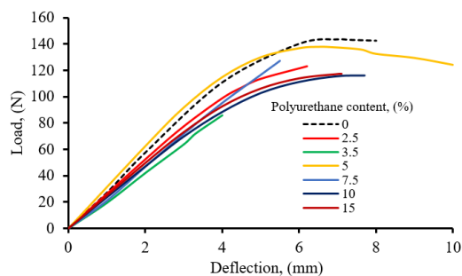
Figure 4. Load-deflection curves of epoxy blends with different amounts of polyurethane
