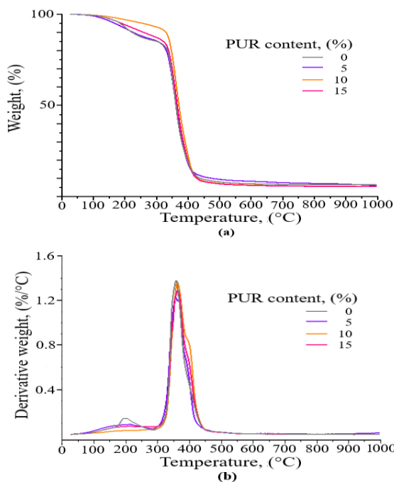
Figure 10. TGA (a) and dTG (b) thermograms
