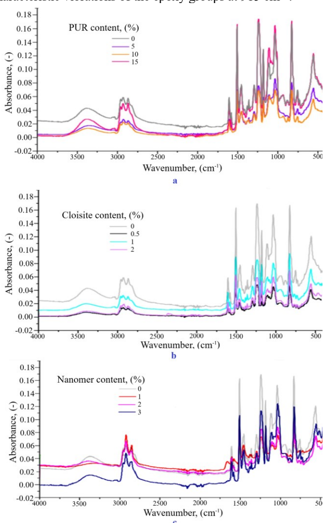
Figure 12. FTIR spectra of epoxy resin and its blends with polyurethane (fig. 12a), nanocomposites with Cloisite (Fig. 12b) and nanocomposites based on Nanomer (Fig. 12c)
