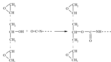
Figure 2. Reaction between the epoxy and polyurethane reactive groups
