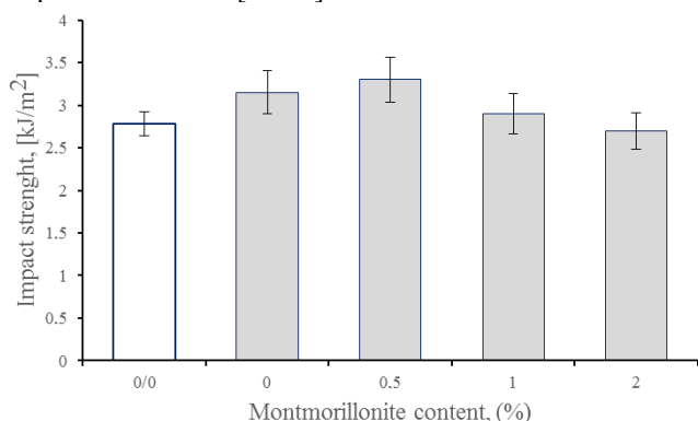
Figure 7. Effect of Cloisite nanoclay content on impact strength of hybrid epoxy matrix modified with 1 wt% Nanomer
