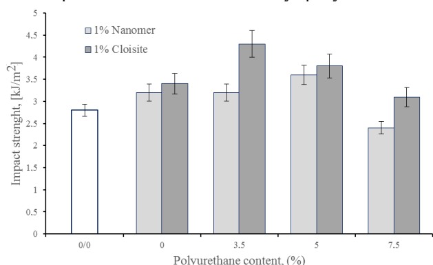
Figure 1. Effect of polyurethane content on impact strength of epoxy resin modified with Nanomer or Cloisite
