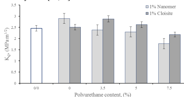
Figure 5. Effect of polyurethane content on the critical stress intensity factor ( K_{IC} ) of epoxy resin modified with Nanomer or Cloisite
