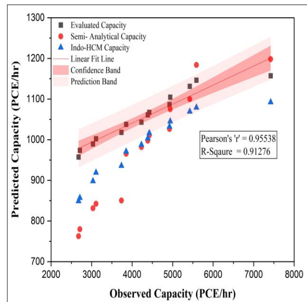
Fig. 6 Comparative analysis of observed and predicted capacities
