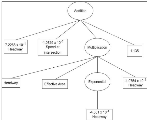
Fig. 5 Tree based structure of OSGP regression model
