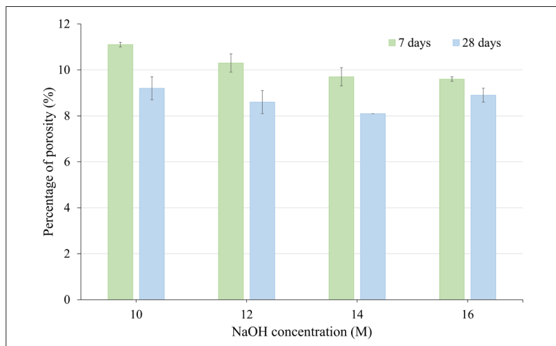
Fig. 2. Percentage of porosity of cold-pressed geopolymer with different NaOH concentration after 7 and 28 days
