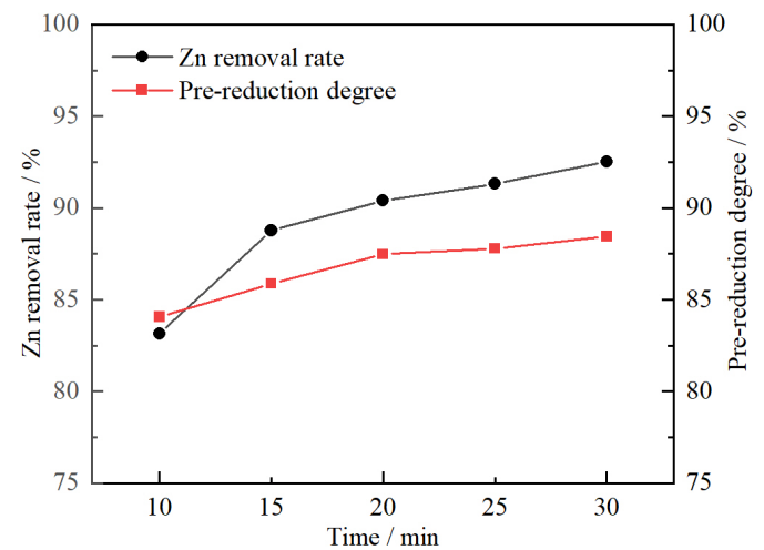
Fig. 6. Effect of pre-reduction time on Zn removal rate and pre-reduction degree of pre-reduction sintered products
