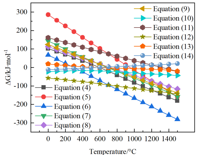
Fig. 9. Standard free energy changes for the Eqs. (4)-(14) in the temperature range of 0 - 1500^\circ\text{C}
