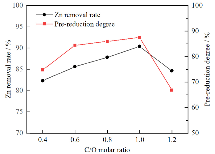
Fig. 4. Effect of carbon content on Zn removal rate and pre-reduction degree of pre-reduction sintered products
