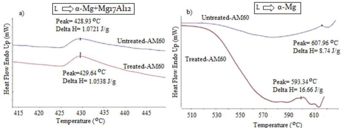
Fig. 4. TG/DTA analysis of the untreated and treated AM60 magnesium alloys; a) 415°C–450°C b) 500°C–610°C
