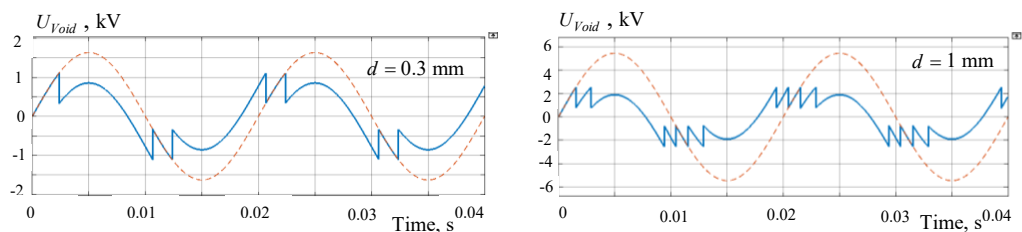
Fig. 5. Results of PD simulation for void diameters d = 0.3 and 1 mm
