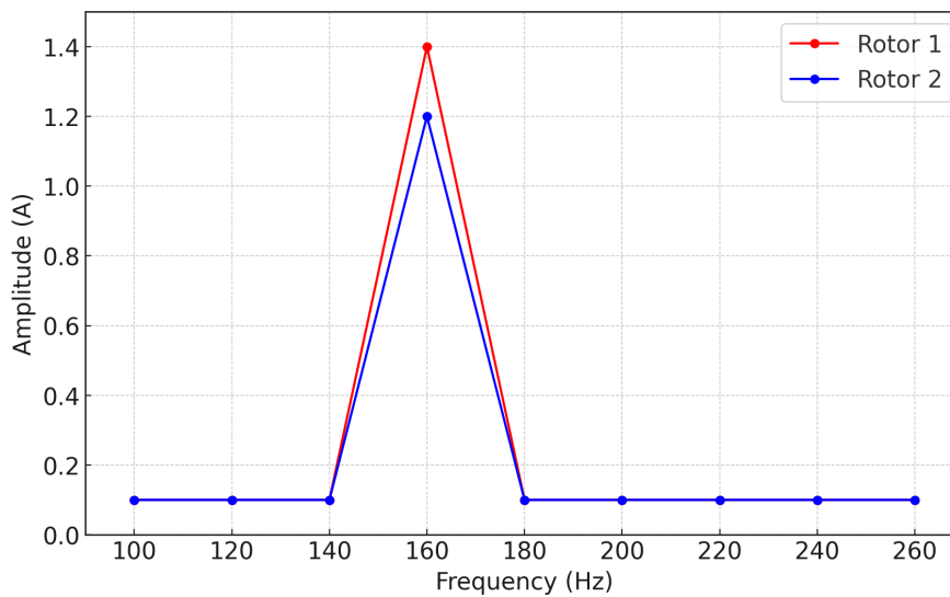
Fig. 6. Stator current of the motor with Rotor1 & Rotor 2
