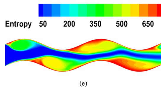
Fig. 7. Entropy contours at 1200 G and Re = 100 for (a) Case 1, (b) Case 2, (c) Case 3, (d) Case 4, and (e) Case 5
