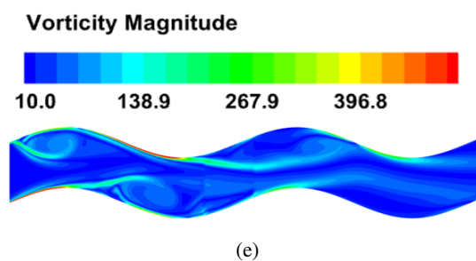
Fig. 8. Vorticity contours at 1200 G and Re = 100 for (a) Case 1, (b) Case 2, (c) Case 3, (d) Case 4, and (e) Case 5
