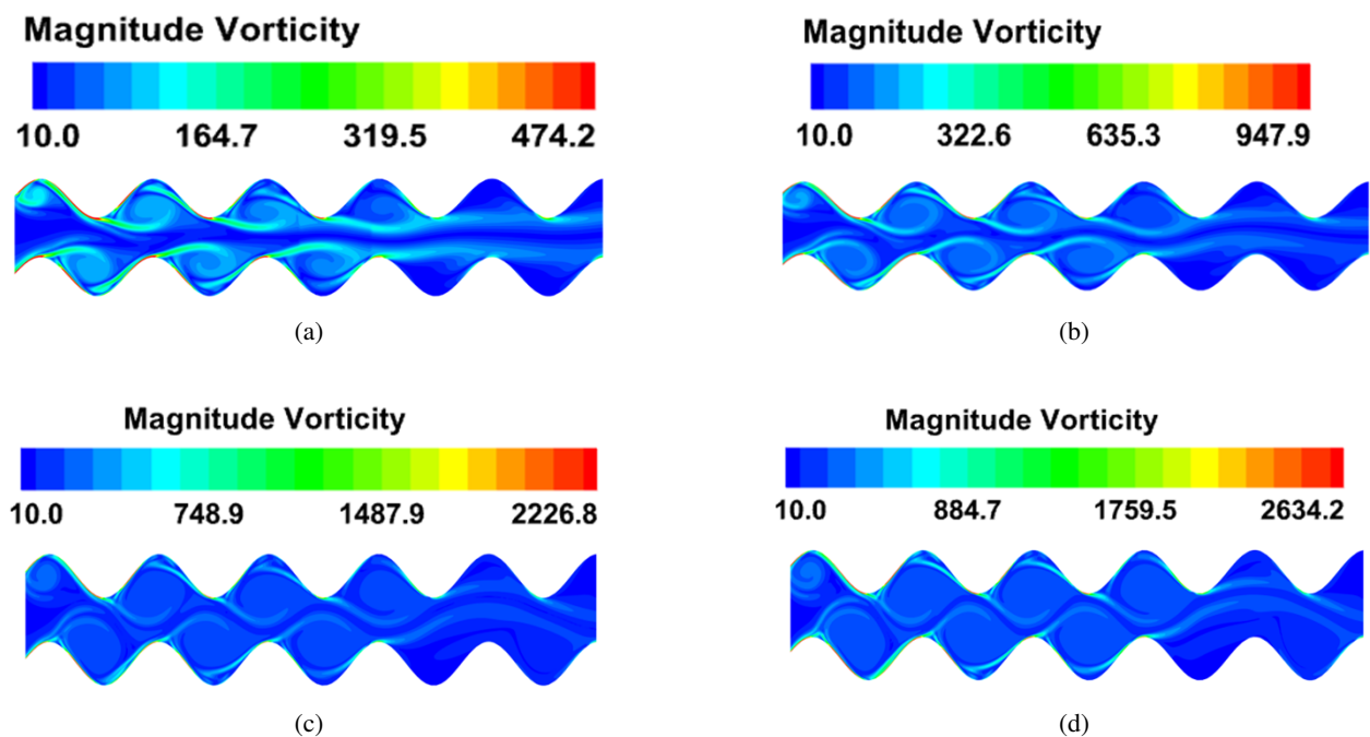
Fig. 6. Vorticity contours for Case 1 and Re = 100 at (a) 1200 G, (b) 1500 G, (c) 2000 G, and (d) 2500 G
